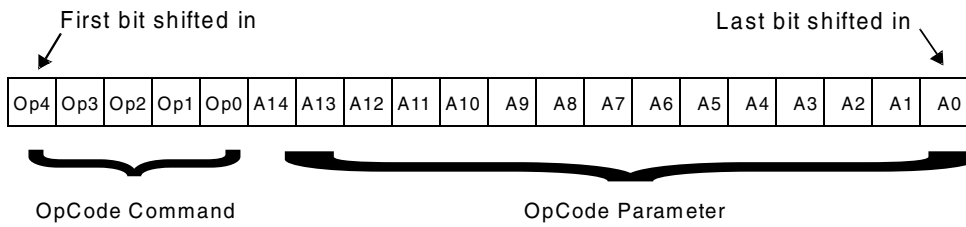
Figure 5 OpCode Format
